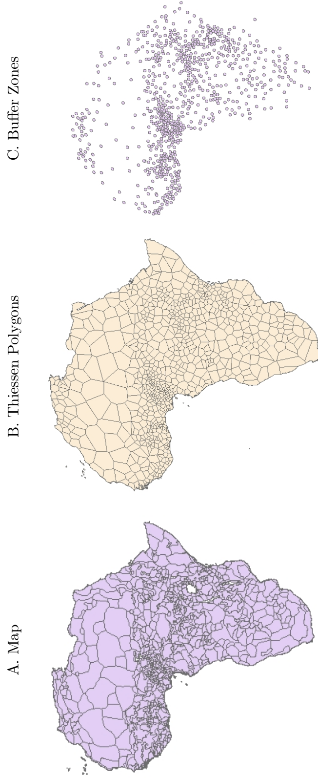
Figure V: Thiessen Polygons
