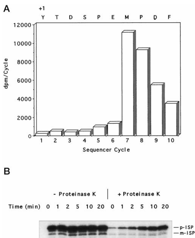
FIG. 8. Determination of the amino terminus of the mature iron-sulfur protein of S. pombe and import into mitochondria of iron-sulfur protein with amino acid changes at positions -2 and -3 from the amino terminus of the mature protein. In panel A, mature iron-sulfur protein of S. pombe was subjected to radiosequencing after in vitro import of [ 35 S]methionine-labeled protein as described under "Experimental Procedures." +1 marks the amino terminus of the mature protein. The radioactivity in samples 8–10 is due to trailing from sample 7 and declines exponentially as expected. In panel B, S. pombe iron-sulfur protein in which Ile-41 and Arg-42, at the -2- and -3-positions relative to the mature amino terminus, had been changed to glycines (pJN92, see Fig. 1) was imported into S. pombe mitochondria.
